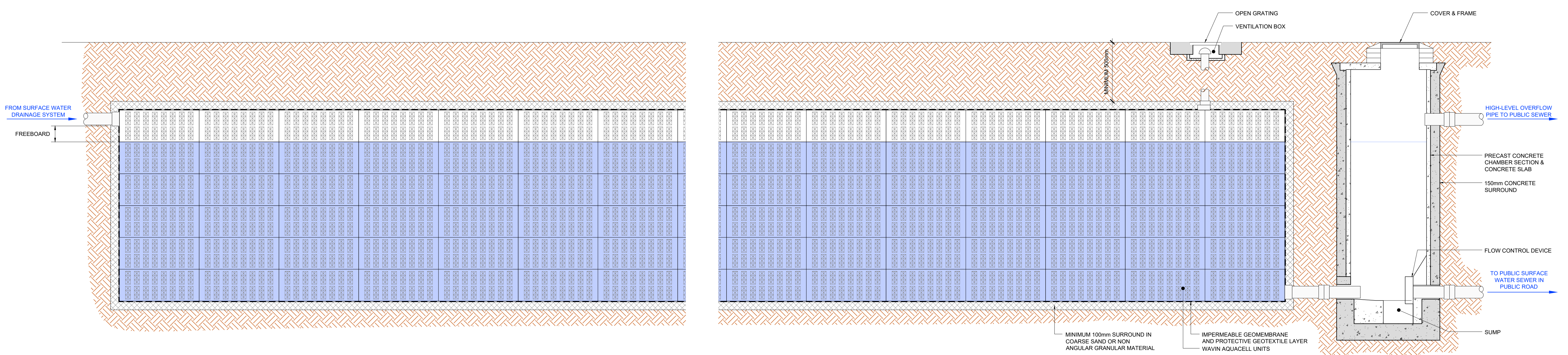
1 SECTION THROUGH WAVIN AQUACELL ATTENUATION TANK (ON-LINE SYSTEM) SCALE 1:25
