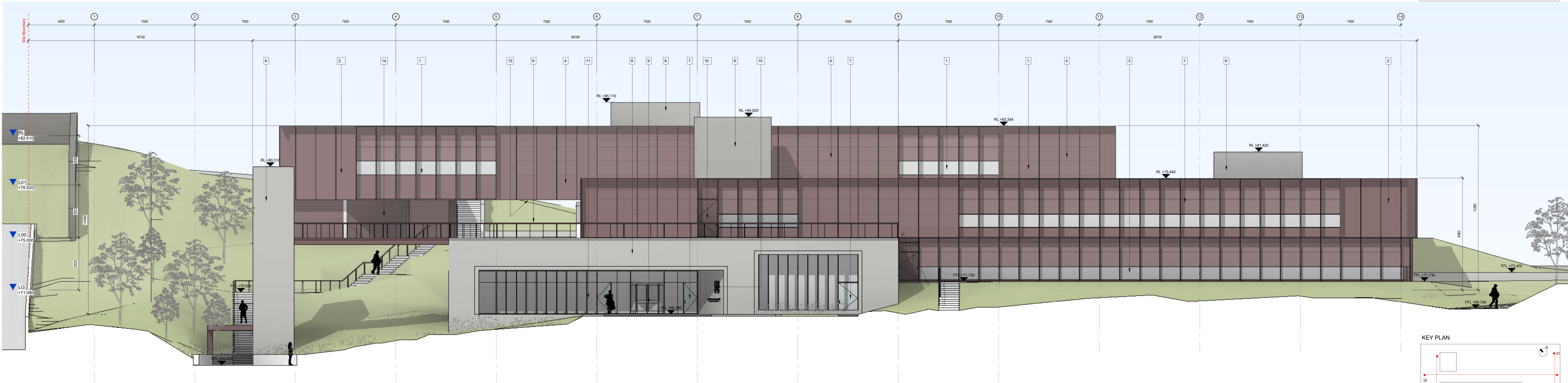
1 GA ELEVATION - SOUTH / WEST 1:100
