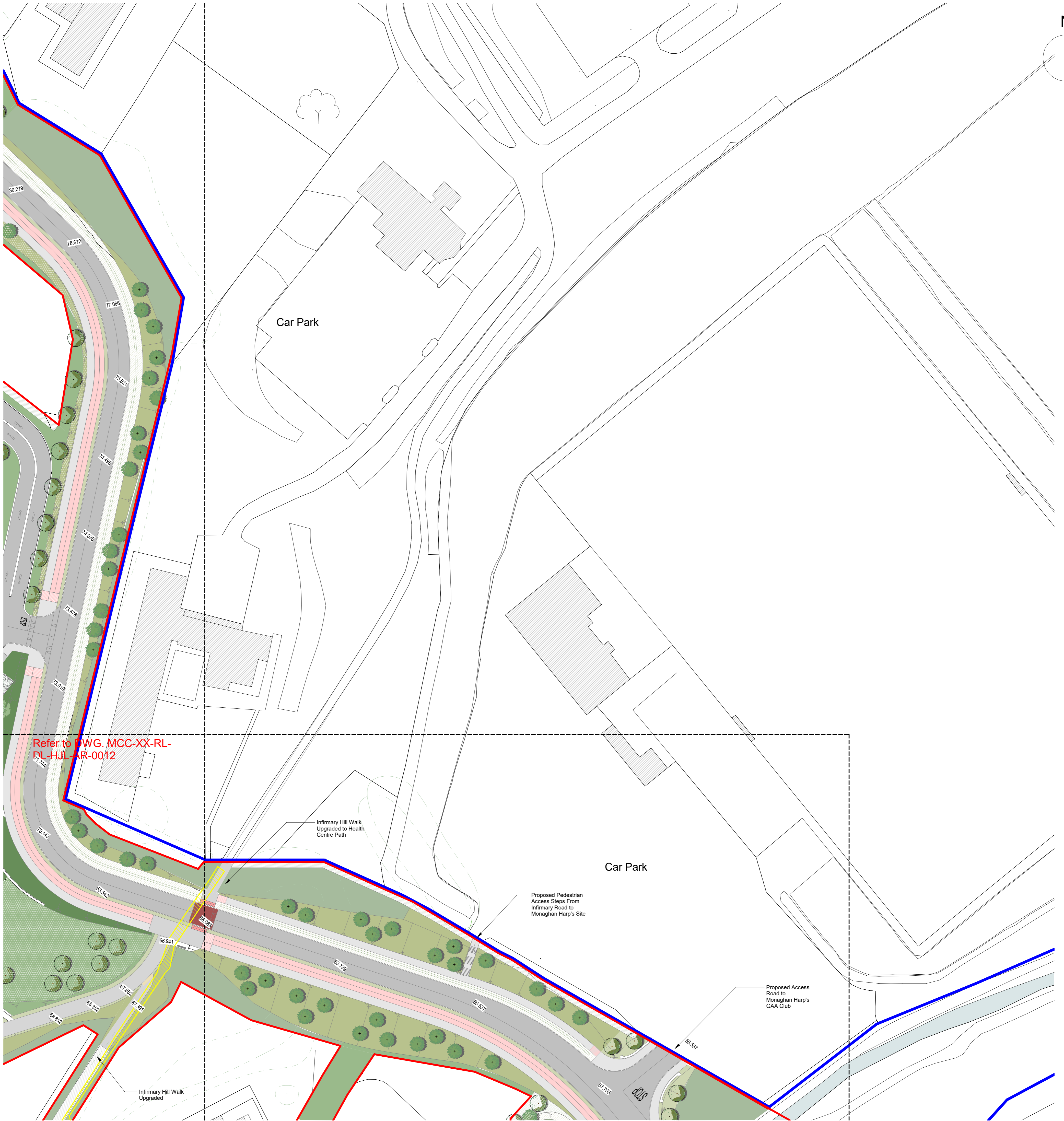
1 PROPOSED SITE LAYOUT PLAN - 2 OF 3 1:500
